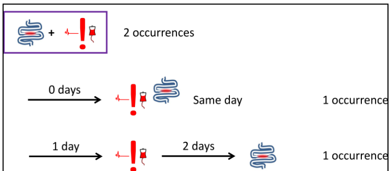
Figure 2. Example of representation of all possible sequences of morbidities (not based on actual data).
