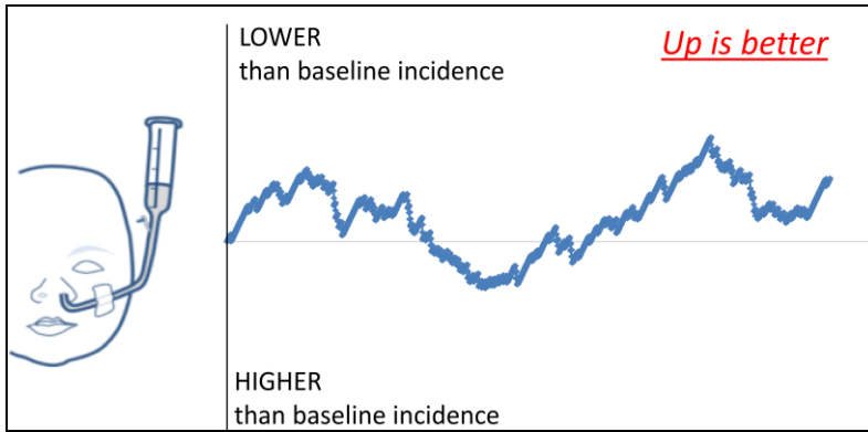
Figure 3. Example of VLAD-style chart (not based on actual data). The incidence of feeding problems seems to be, on average, in line with the compared benchmark (baseline incidence) but with an interesting cyclic trend where periods characterised by an incidence lower than the baseline alternate with periods characterised by an incidence higher than the baseline.
