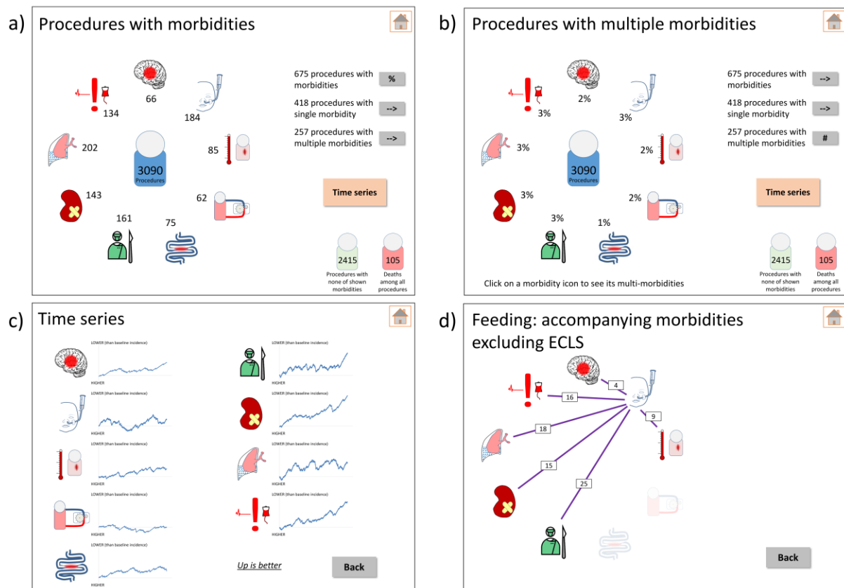
Figure 4. Examples of slides included in the output presentation (not based on actual data).
